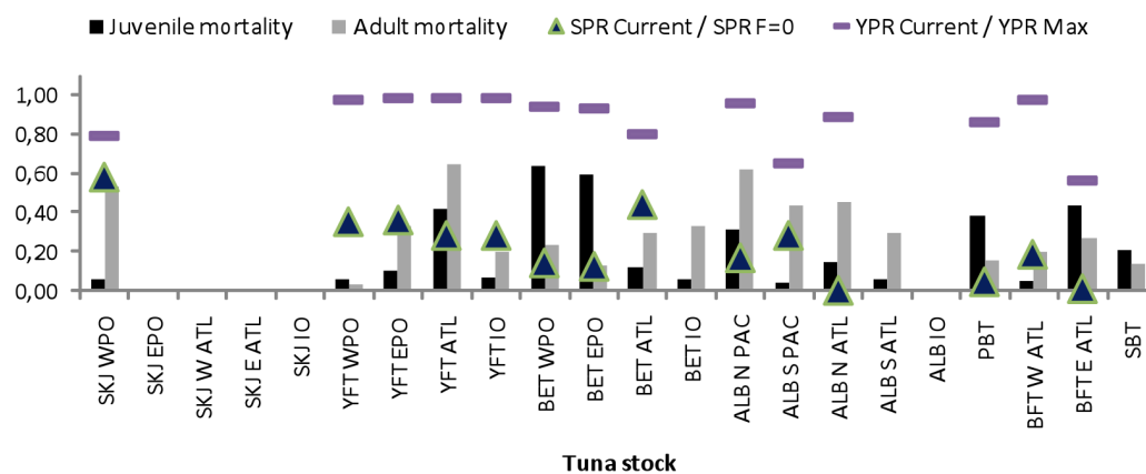
Figure 8. Average juvenile and adult fishing mortality at age (year -1 ) in the last period of one generation in relation to current spawning-per-recruit ratio ( SPR_{current}/SPR_{F=0} ) and yield-per-recruit ratio ( YPR_{current}/YPR_{Maximum} ).
