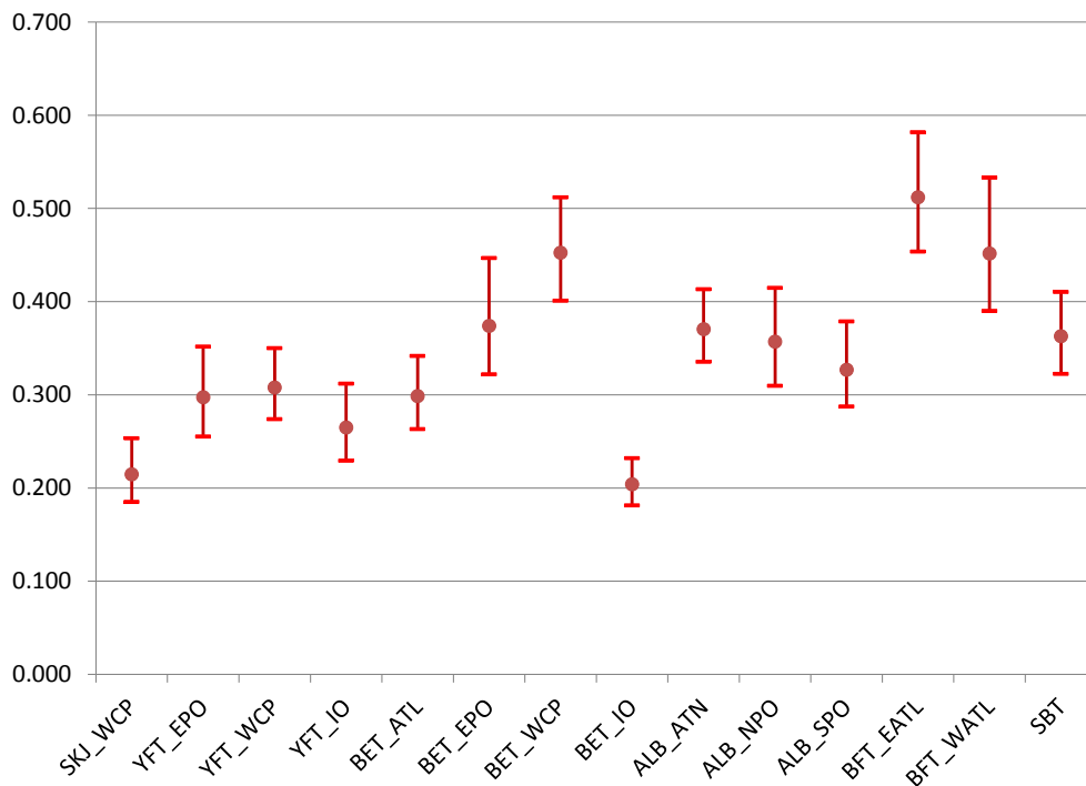
Figure 5. Preliminary results of the first meta-analysis showing \sigma_R for different stocks of tunas. NOTE: all data and analyses are preliminary.
