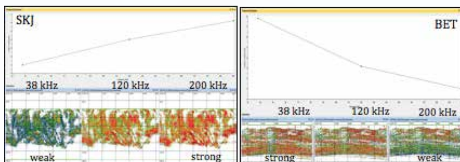
Fig 3. Example of frequency response of skipjack (non-swimbladdered fish, left) and bigeye (swimbladdered fish, right) tunas during the survey.
