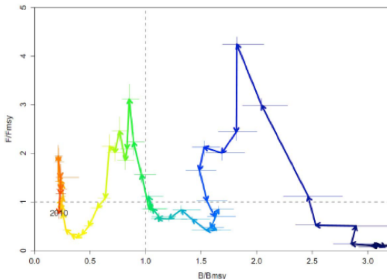
Figure SH-2. Temporal trend in the median ratios B_{\text{current}}/B_{\text{MSY}} (x-axis) and F_{\text{current}}/F_{\text{MSY}} (y-axis) for southern bluefin tuna. Vertical and horizontal lines provide an idea of the relative uncertainty in the estimates. Colors are taken from CCSBT reports and do not necessarily correspond to the colors used for ratings in the ISSF Stock Status Report.
